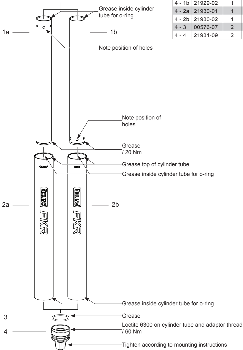
Figure 4 - Cylinder tube assembly
