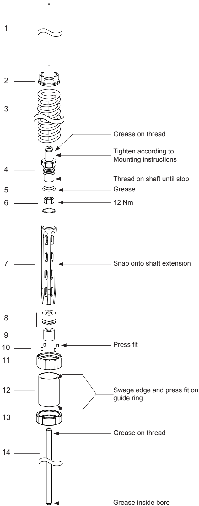
Figure 2 - Shaft assembly
